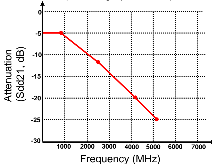
Attenuation Limit (for Category 2 Non Equalized Cable)
